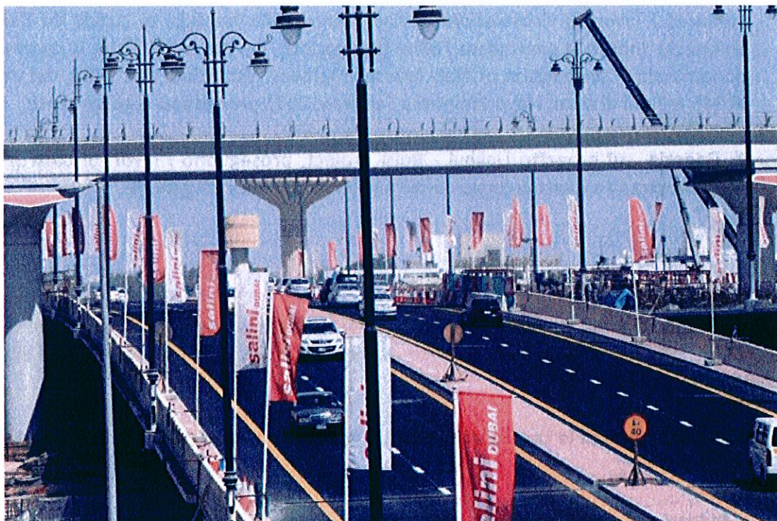
Dubai, Ras Al Khor Crossing
